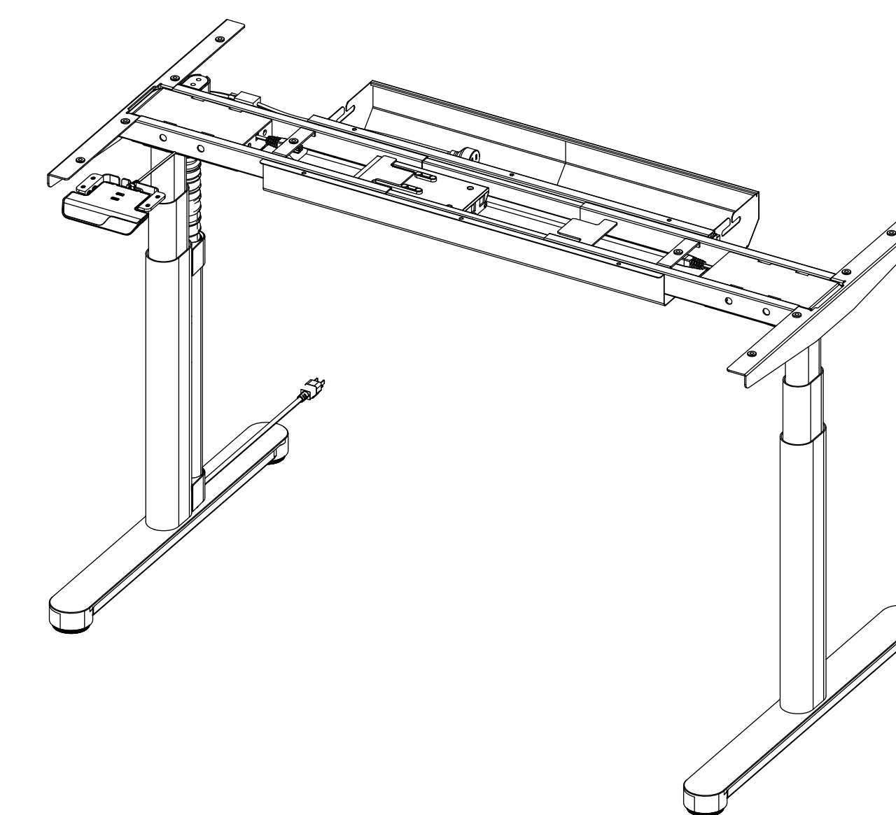
3-D View
